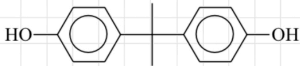
bisfenol A
